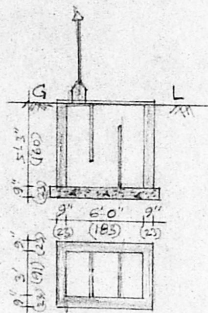
SEPTIC TANK
